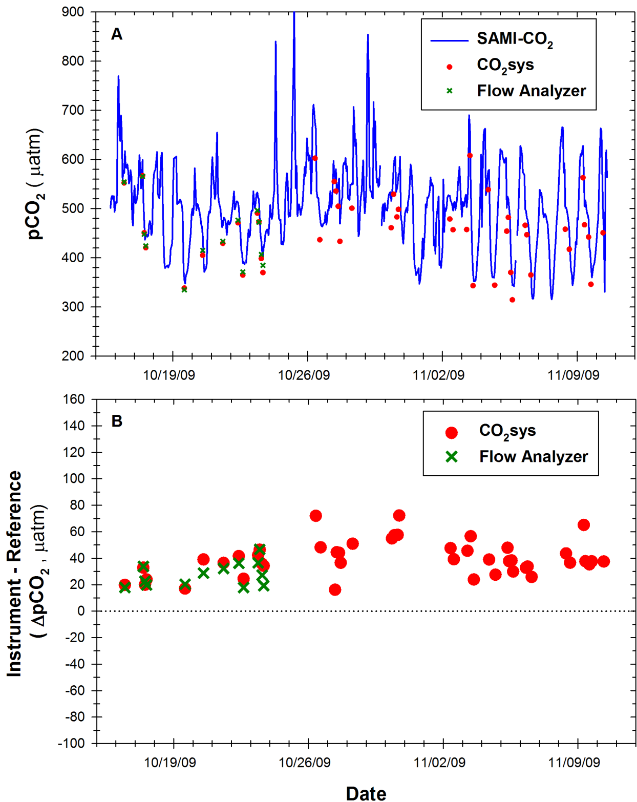
Figure 7. Field data from of the Sunburst SAMI- \text{CO}_2 p\text{CO}_2 instrument during deployment in Kaneohe Bay, HI. Panel A: Time series of instrument values (blue lines) with overlaid values from two reference samples, one from a Flow Analyzer (green X) and the other based on calculations from pH and total alkalinity measurement using \text{CO}_2\text{Sys} (red dot). Panel B: The difference between instrument values and reference values. Dotted line represents perfect agreement or zero difference. Reference data symbol size is scaled to 8 \mu\text{atm} , corresponding to the uncertainty in the reference, see text for explanation.
