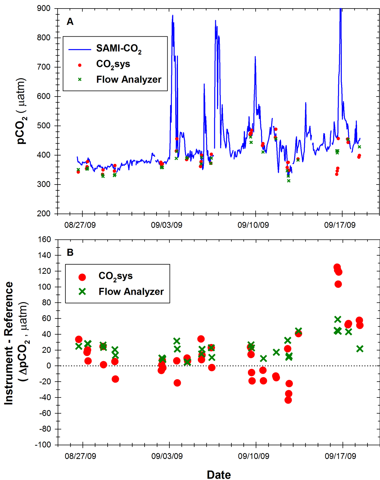
Figure 3. Field data from the Sunburst SAMI-CO 2 pCO 2 instrument during deployment in Hood Canal, WA. Panel A: Time series of instrument values (blue lines) with overlaid values from two reference samples, one from a Flow Analyzer (green X) and the other based on calculations from pH and total alkalinity measurement using CO 2 Sys (red dot). Panel B: The difference between instrument values and reference values. Dotted line represents perfect agreement or zero difference. Reference data symbol size is scaled to 8 µatm, corresponding to the uncertainty in the reference, see text for explanation.
