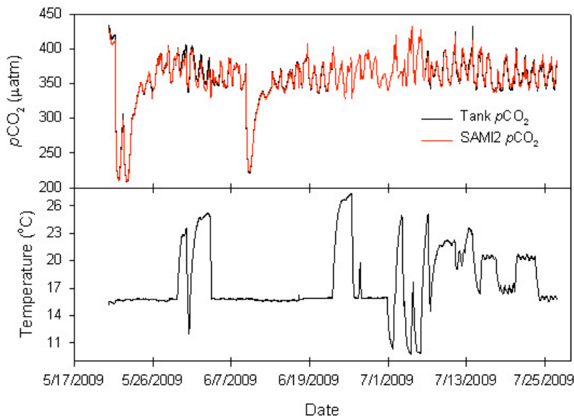
Figure 1: SAMI- \text{CO}_2 tank data tracked against calibrated Licor 840 over almost 3 month period.
