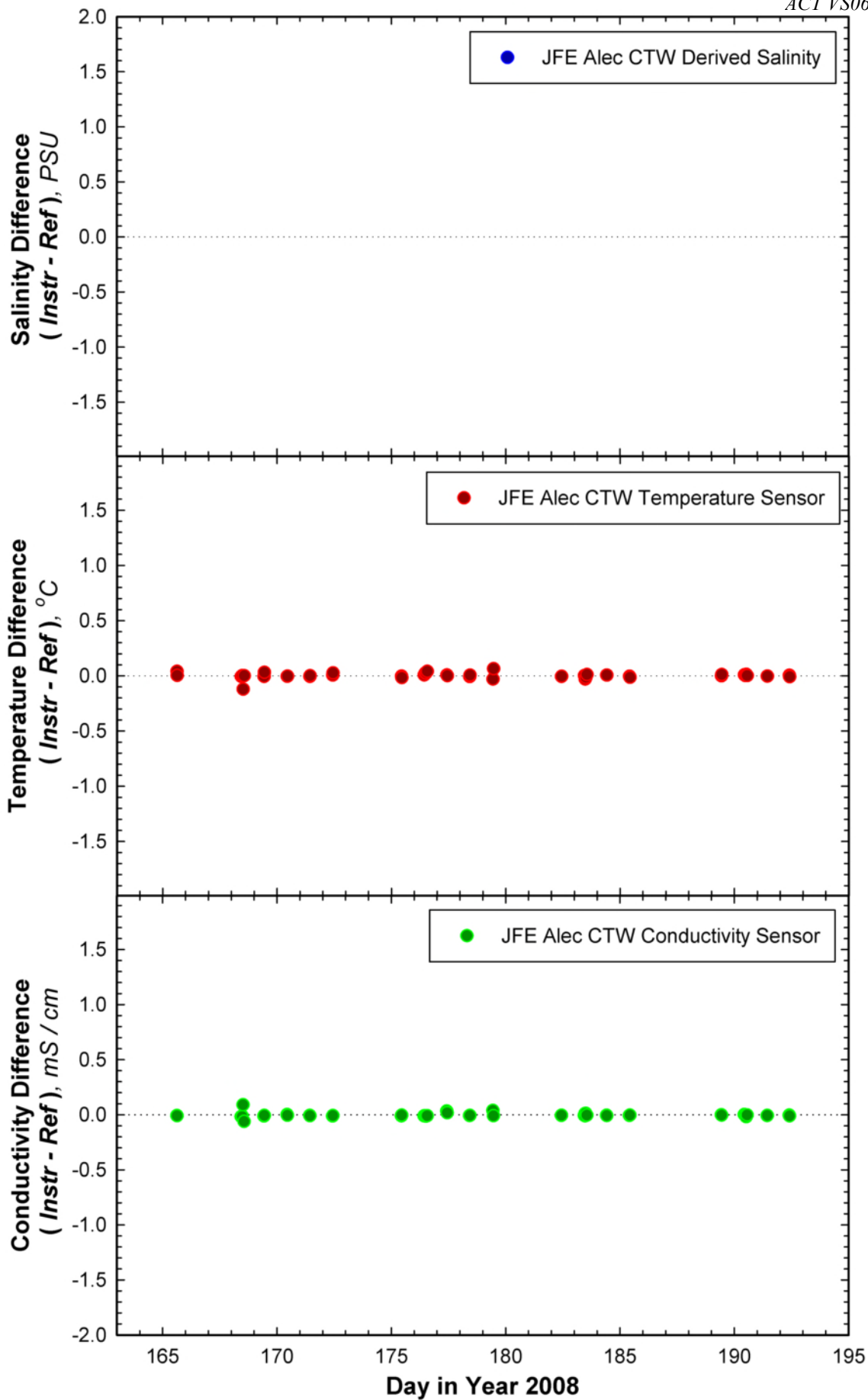
Figure 26. Assessment of relative accuracy of instrument time series measurements during GL field deployment.
