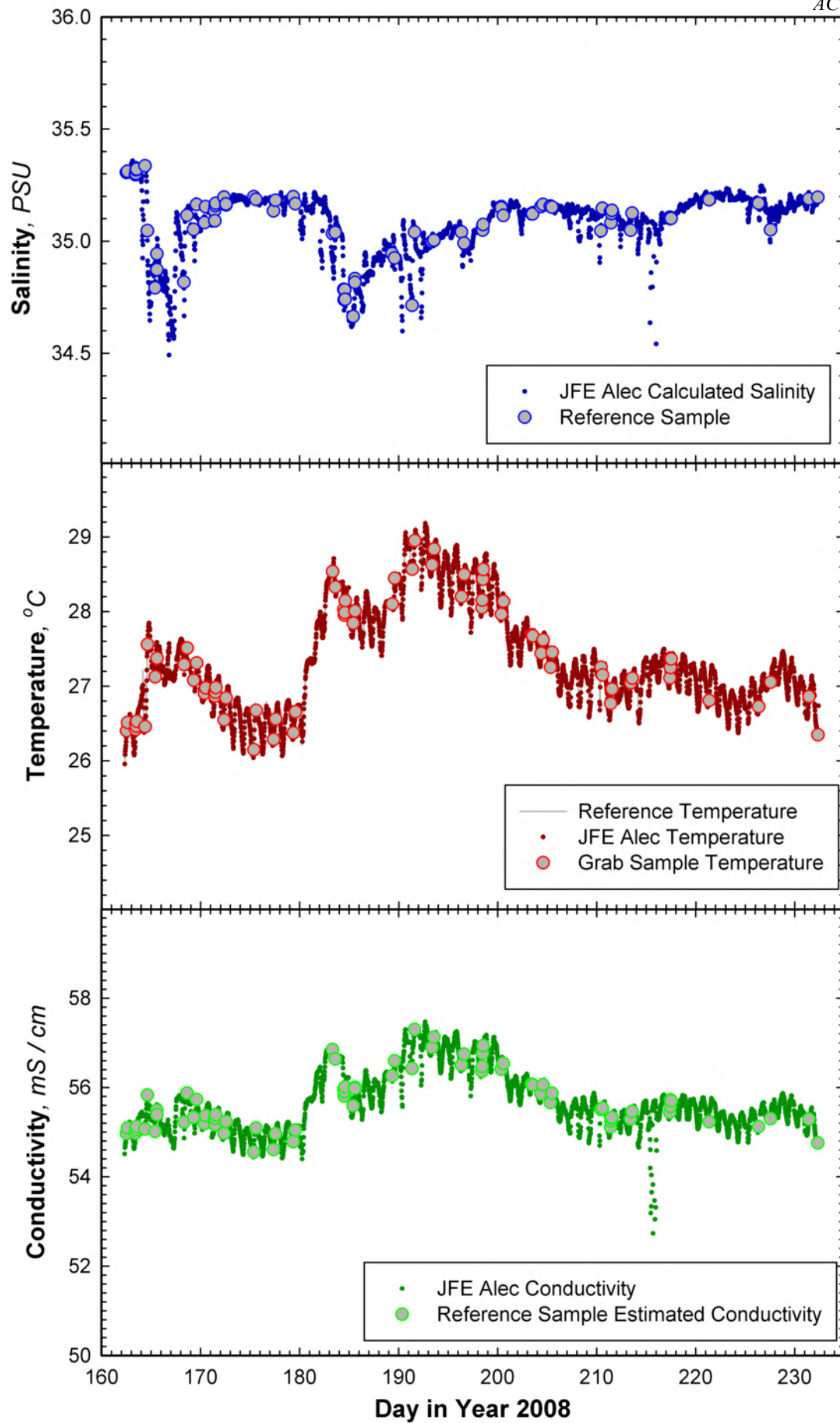
Figure 19. Time series of instrument measurements and corresponding reference samples acquired during HI field deployment.
