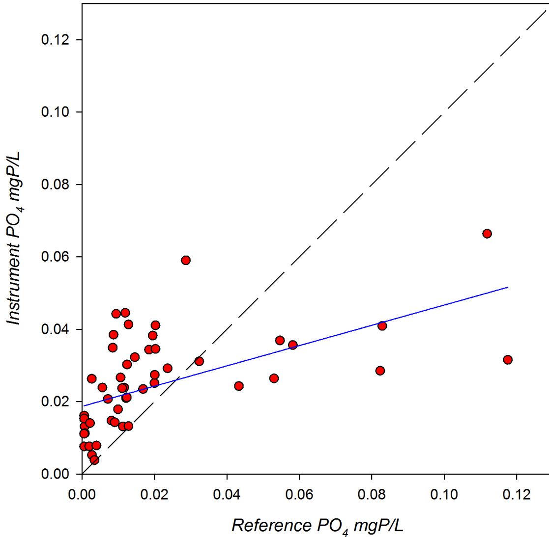
Figure 11. Maumee River field response plot for the 32 day deployment of the Systea-PO 4 compared to reference PO 4 samples. The plotted line represents a 1:1 correspondence, the blue line represents the linear regression.
