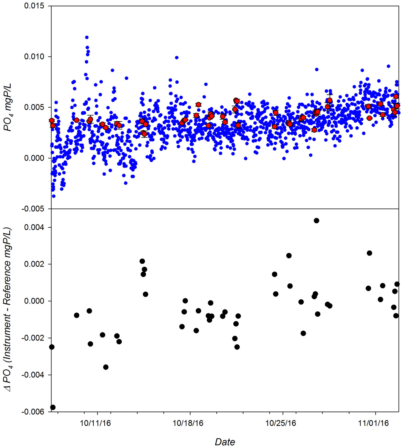
Figure 20. Top panel: Time series of PO 4 measured by the Systea-PO4 deployed during the one month HIMB field trial. Continuous PO 4 recordings from instrument (blue dots) and PO 4 of adjacent grab samples (red circles.) Bottom Panel: Time series of the difference between the Systea-PO4 and reference measurements for each matched pair (Instrument mgP/L – Reference mgP/L).
