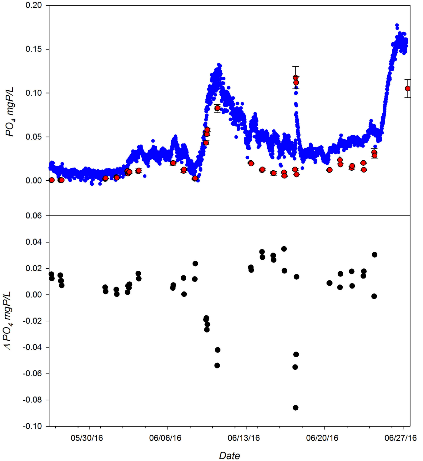
Figure 10. Top Panel: Time series plot of the Systea-PO 4 measurement (blue dots) and reference measurements (red dots) of phosphate in mgP/L. Bottom Panel: Time series plot of the difference between the Systea-PO 4 and reference measurements of phosphate in mgP/L (instrument – reference) during the freshwater deployment in the Maumee River at Waterville, OH.
