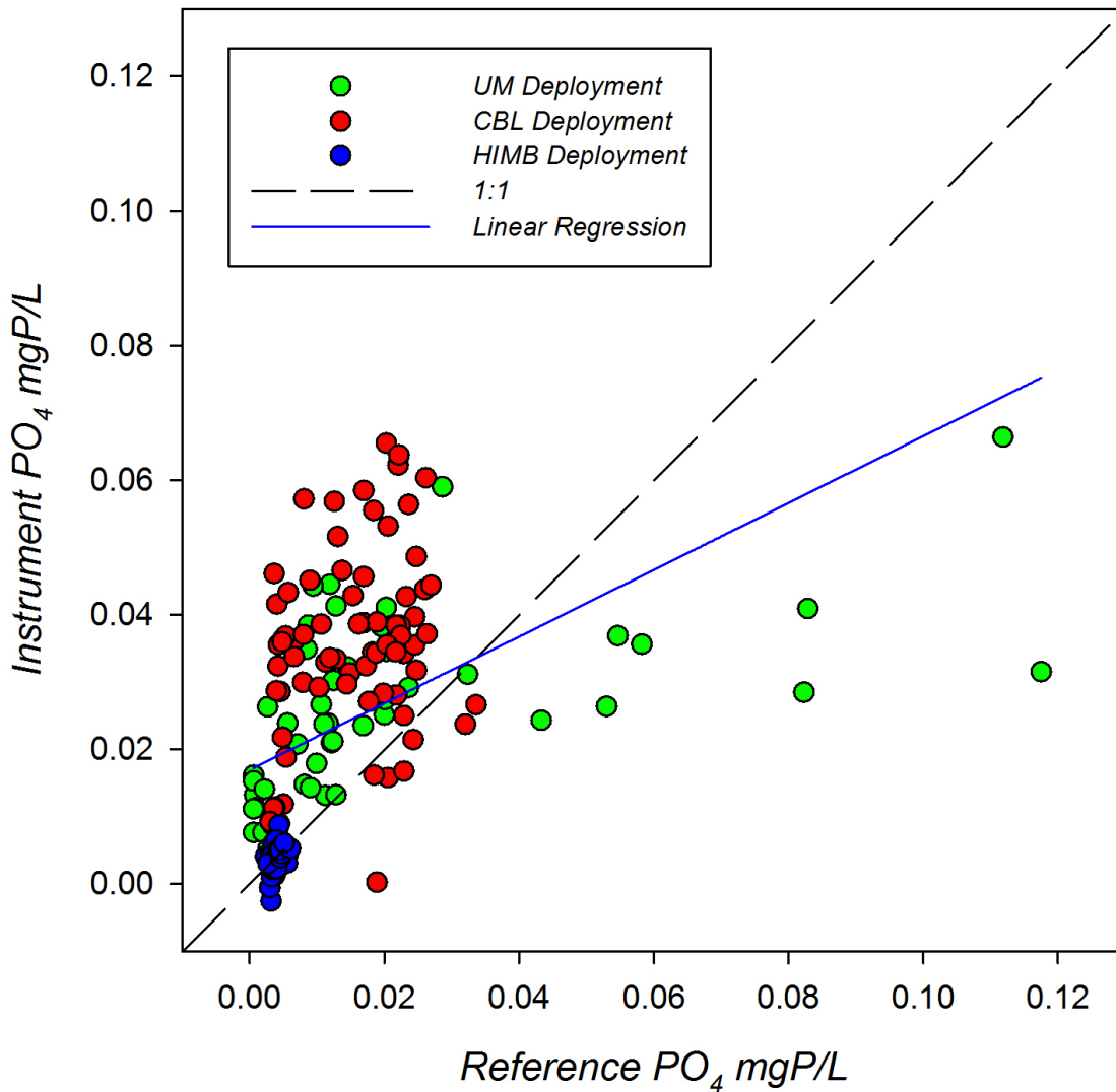
Figure 23. Global response plot for the Systea-PO4 observed during the three ACT field trials. Black dotted line represents a 1:1 correspondence, the blue line represents the linear regression.
